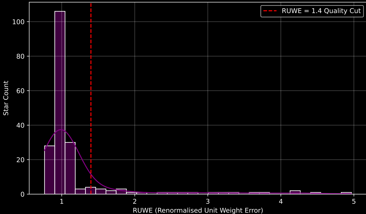
GAPOGEE DR17 Field [098+63_MGA] RUWE Distribution (n= 194)
