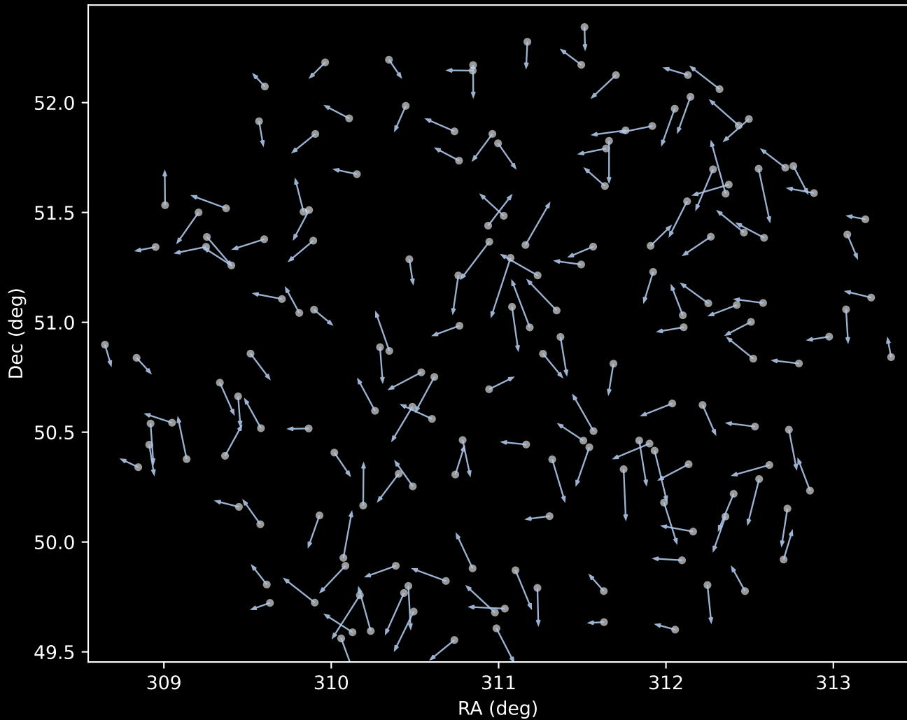
APOGEE DR17 Cluster 1 Proper Motion Vectors (n=168)
