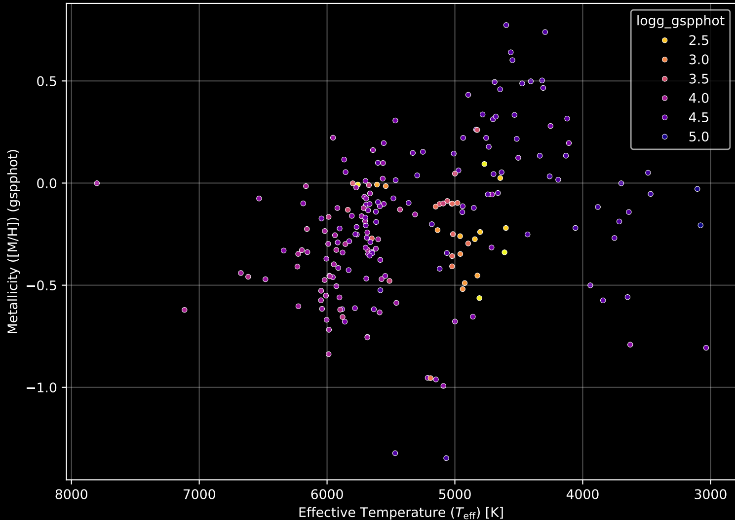
APOGEE DR17 Field: [098+63_MGA] Stellar Population Parameters (n= 209)
