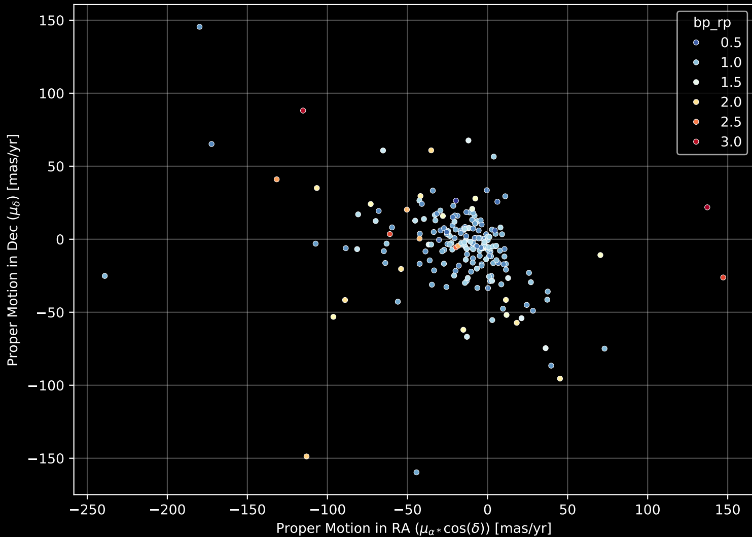
APOGEE DR17 Field: [098+63_MGA] Proper Motion Diagram (n= 209)
