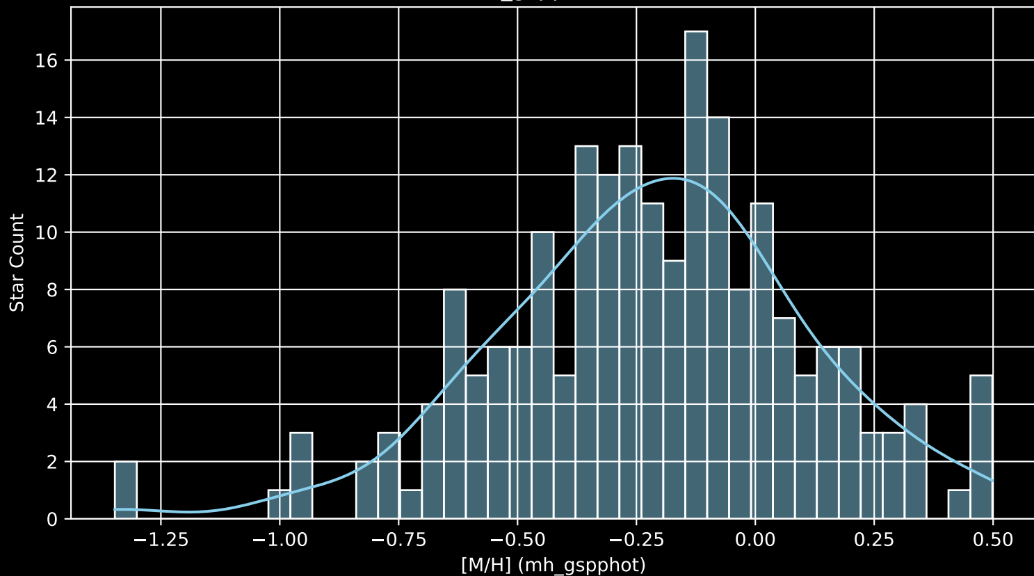
APOGEE DR17 Field: [098+63_MGA [M/H] (mh_gspphot) (n= 204)
