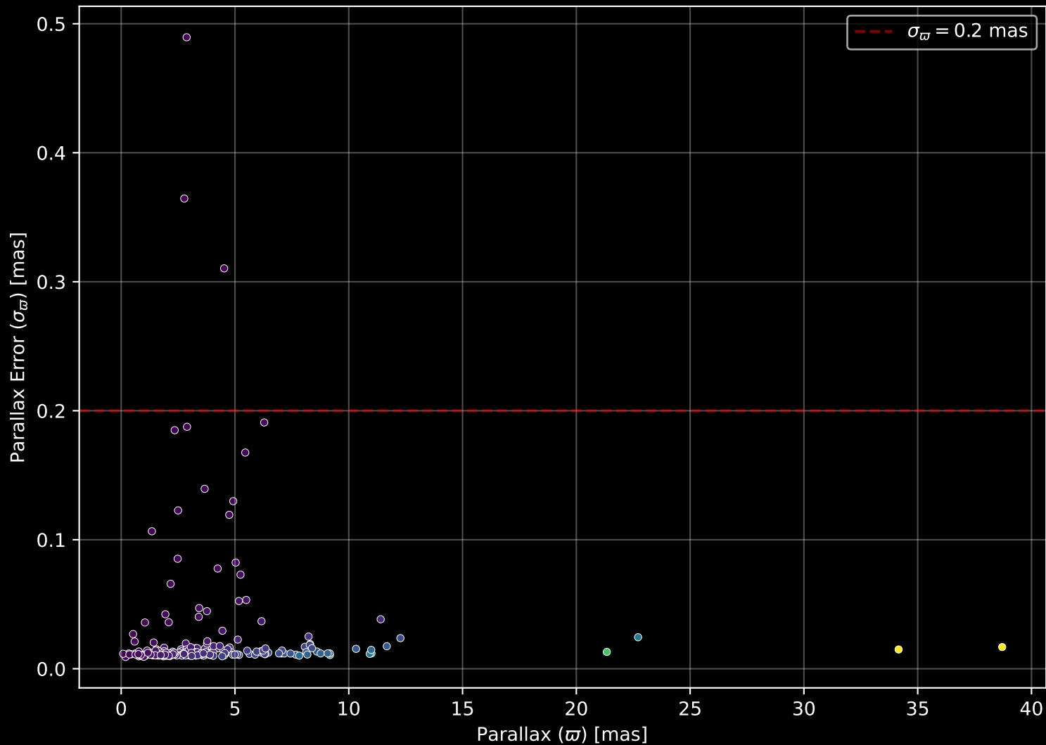
APOGEE DR17 Field: [098+63_MGA] Parallax Quality (n= 209)
