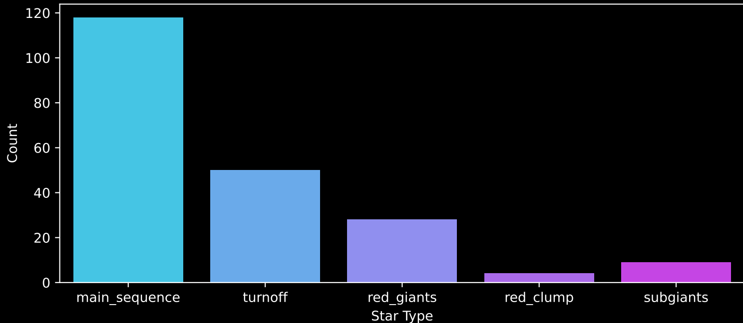
APOGEE DR17 Field: [098+63_MGA] Count plot of Star Type
